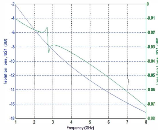
Fig.3:-Expected result of simulation parameters like Isolation loss and insertion loss versus Frequency of switch in on- and off state.
