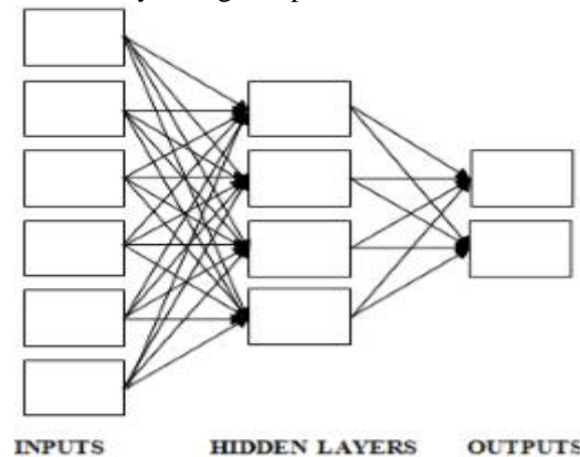
Fig 1 Feed-forward network model
