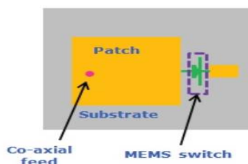
Fig 2.Schematic layout of RF-MEMS Switch with reconfigurable antenna.
